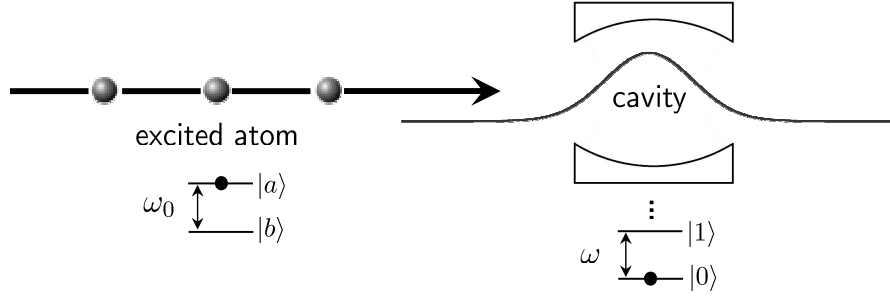
FIG. 1 – Micromaser pumped by two-level atoms.
